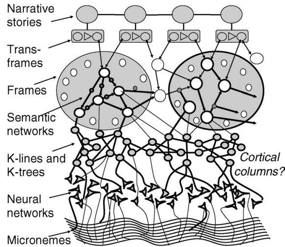
FIGURE 38.11. The structures we can use at different levels to represent objects and ideas. Adapted from Minsky (2006).
